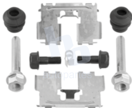
KIT DE CALIPER RUEDA TRASERA TOYOTA CAMRY (07-17), RAV4 (02-09) 8332 D1212.
