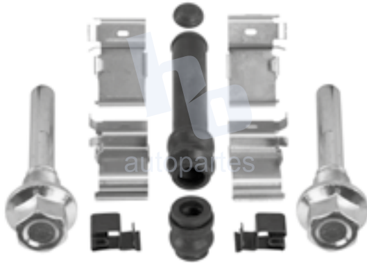
KIT DE CALIPER RUEDA DELANTERA TOYOTA HILUX 4X2 (89-95), LONG BED XTRA CAB (92-93), PICKUP (92-95) 7320 D589, TACOMA (95-04) 7320 D589, 7320 D433.
