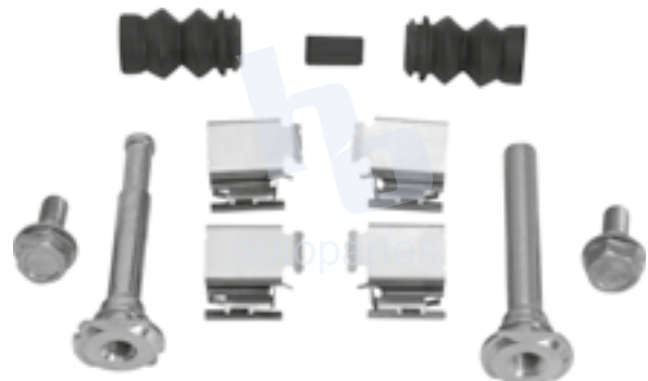
KIT DE CALIPER RUEDA DELANTERA PEUGEOT 206 (03-07) 775Y F222, 8779 D1570, PEUGEOT 208 (14-15) 775Y F222, RENAULT MEGANE II (05-08) 7Y21 F256, SCENIC (05-08) 8779 D1495.
