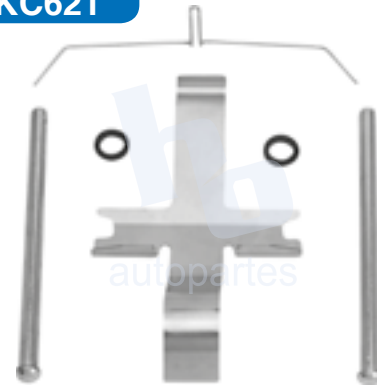
KIT DE CALIPER RUEDA DELANTERA TOYOTA 4RUNNER (92-01), HILUX 4X4 (84-97), LAND CRUISER (91-98), PICKUP 1/2 TON 4X4 (98-05) 7298 D611, PICKUP T100 WD (93-95) 7298 D436, 7298 D611, PRADO (82-01), RAV4 (98-05), TACOMA (95-04), TACOMA 4WD (95-97) 7298 D611.
