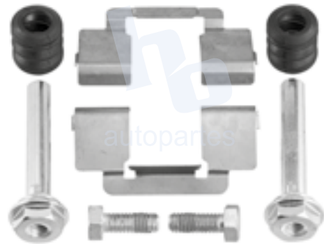
KIT DE CALIPER RUEDA DELANTERA RENAULT CLIO SPORT (06-07) 8779 D1570, MEGANE (5), SCENIC (4) 8695 D1495, 7Y01 F207.
