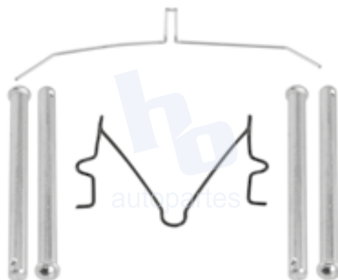
KIT DE CALIPER RUEDA DELANTERA TOYOTA 4RUNNER (84-88), HILUX (79-88), LAND CRUISER (75-86) 7069 D137.
